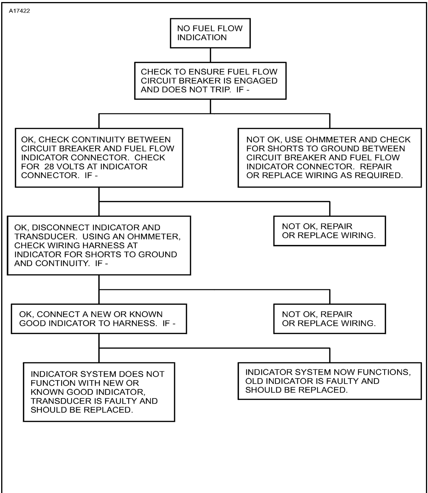
Figure 101 : Sheet 1 : Fuel Flow Indicator Troubleshooting Chart
